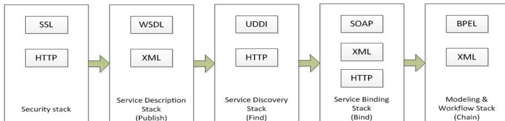
Figure 1. Web service standards of standard service environment
