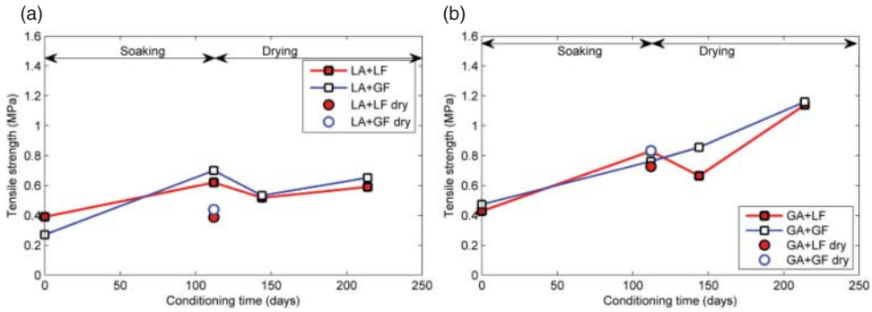
Figure 15. Effect of moisture conditioning at 20°C on cohesive strength of asphalt mastics. Tensile strength was obtained using a loading rate of 20 mm/min at a temperature of 20°C. (a) Limestone mastics and (b) granite mastics.
