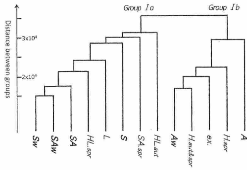
Fig. 4 Dendrogram of clusters (SLP distribution patterns) for the cold season
