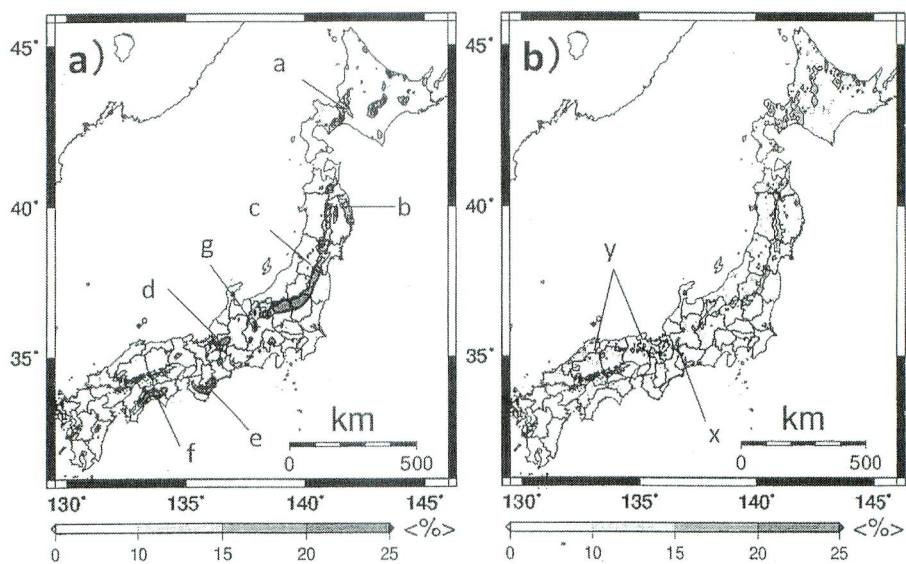
Fig. 2 30-years average of relative frequency (%) for weather divide determined by a) sunshine duration and b) precipitation amount.
