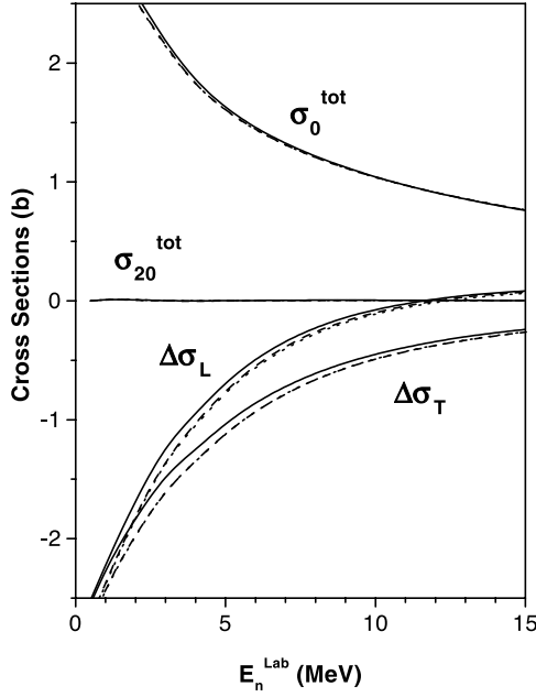
FIG. 1. The total cross sections, \sigma_0^{\text{tot}} , \Delta\sigma_L , \Delta\sigma_T , and \sigma_{20}^{\text{tot}} , of the nd scattering as functions of incident neutron energy in laboratory system for AV18 (solid lines), AV18+BR-3NF (dashed lines), and AV18+GS-3NF (dotted lines). The dashed lines and the dotted ones overlap each other.
