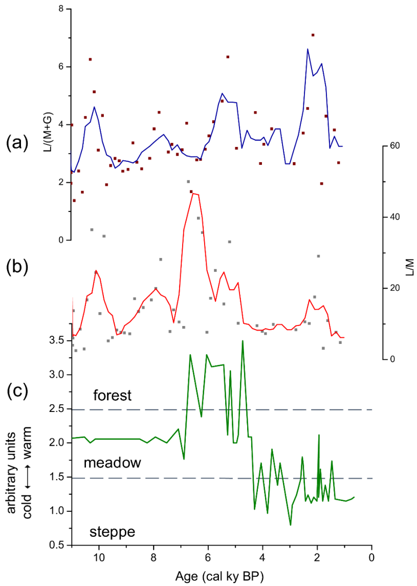
Figure 4: (a) Paru Co L/(M+G) ; (b) Paru Co L/M (trends obtained with a 5-points moving average); (c) Hidden Lake pollen inferred vegetation, data graphically obtained with GetData Graph Digitizer from Tang et al., (2000).
