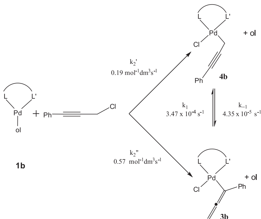
Scheme 6. Reactivity network and related rate constants for the reaction: 1b + Ph-C \equiv C-CH _2 Cl \rightarrow 3b + 4b .
