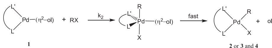
Scheme 4. Schematic representation of the mechanism of the reaction between type 1 complexes and chloropropynes.
