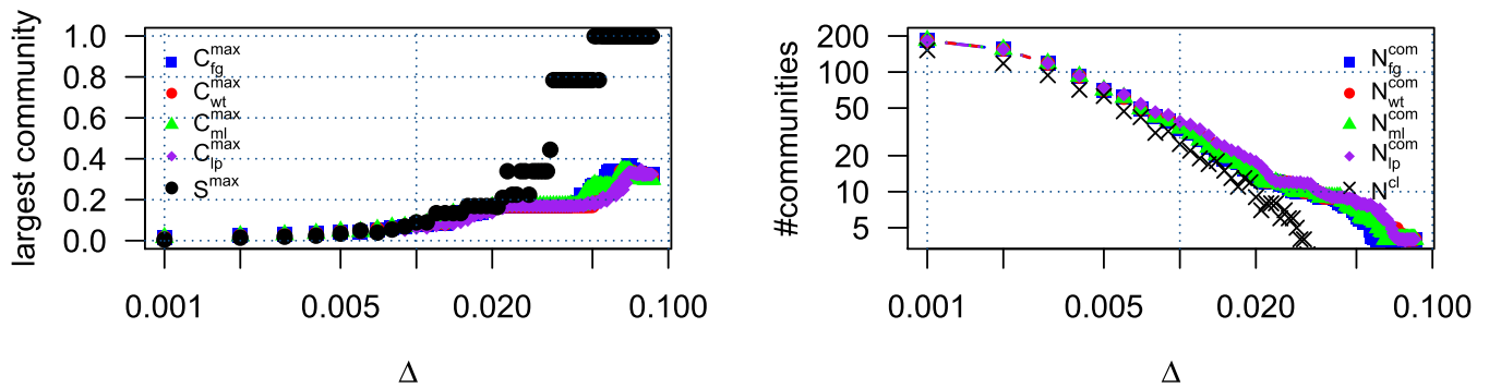
Fig. 5. Analysis of the synthetic pages-to-pages graphs G_{\text{sim}}^p generated according to our extension of the BCM model. (Left) We show the size of the largest component S_{\max} and the size of the largest community |C_{\max}^{\text{alg}}| versus the tolerance \Delta . (Right) We show the number of connected components N_{\text{cl}} and the number of detected communities N_{\text{com}}^{\text{alg}} ; notice that by definition, the number of communities must be N_{\text{com}}^{\text{alg}} \geq N_{\text{cl}} .
