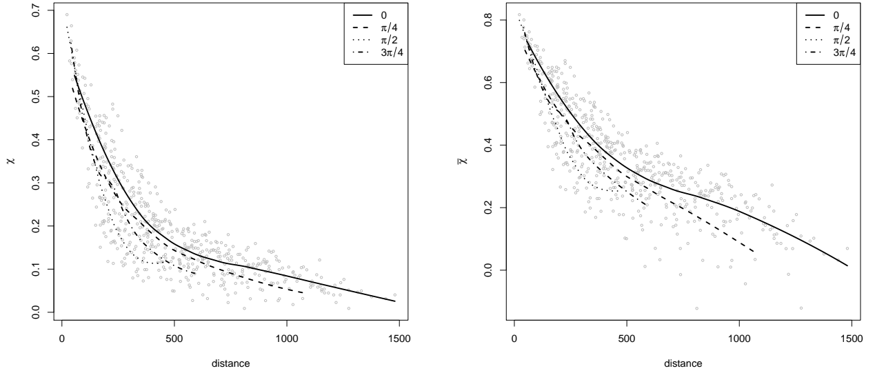
Figure 4: Empirical evaluation of the functions \hat{\chi}(h, u) (left) and \hat{\bar{\chi}}(h, u) (right) at u = 0.975 . Gray circles give empirical value between all available pairs. Lines represent smoothed values of the empirical estimates using the pairs in the directional sectors (-\pi/8, \pi/8] , (\pi/8, 3\pi/8] , (3\pi/8, 5\pi/8] and (5\pi/8, 7\pi/8] .
