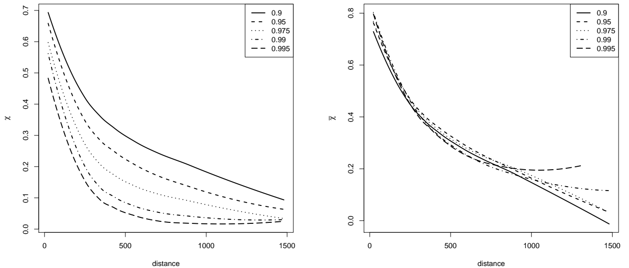
Figure 5: Smoothed values of the empirical estimates of the functions \hat{\chi}(h, u) (left) and \hat{\bar{\chi}}(h, u) (right) at different values of the threshold u .
