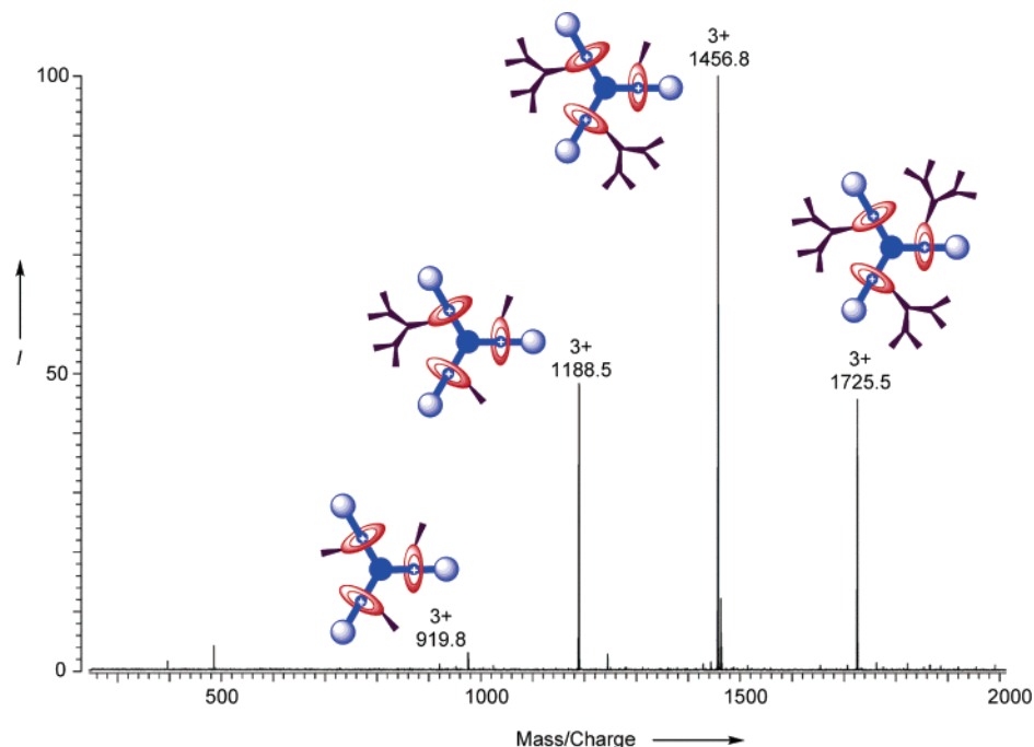
Figure 5. ESI-MS result of the 1:1 mixture of dynamic [G0]-dendrimer 4a-H 3 ·3PF 6 and dynamic [G2]-dendrimer 4c-H 3 ·3PF 6 , indicating the newly formed, mixed-dendron dynamic dendrimers in MeCN.
