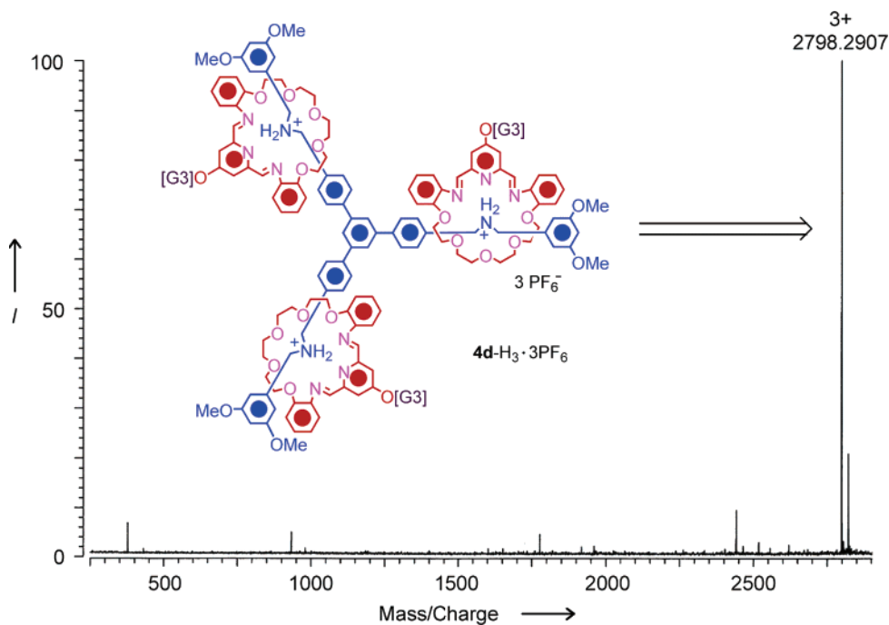
Figure 3. HR-ESI-MS analysis of the dynamic [G3]-dendrimer 4\text{d}\text{-H}_3\cdot 3\text{PF}_6 .
