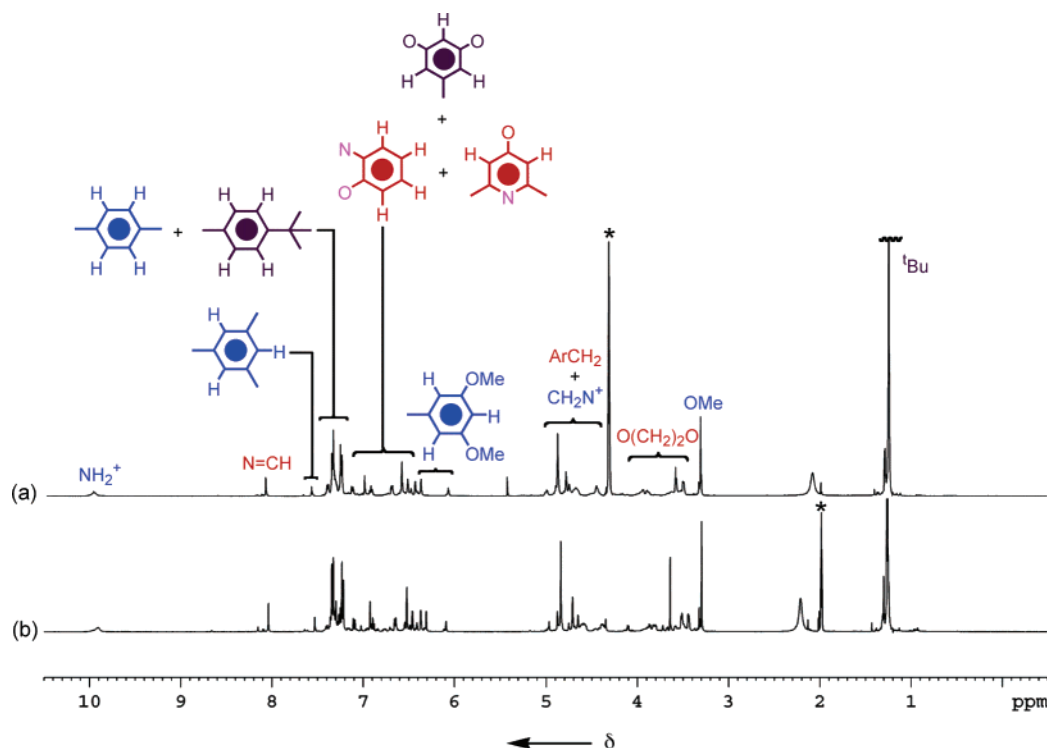
Figure 2. ^1\text{H} NMR spectra (500 MHz, 298 K, 35 mM) of the dynamic [G2]-dendrimer 4\text{c}\text{-H}_3\cdot 3\text{PF}_6 after 20 min of mixing of the appropriate components in (a) \text{CD}_3\text{NO}_2 and (b) \text{CD}_3\text{CN} (* = solvent residue).
