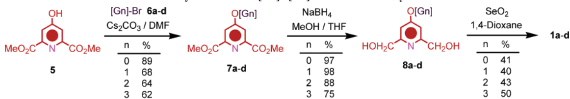
Scheme 2. Synthesis of the [G0]–[G3] Dendritic Dialdehydes 1a–d
