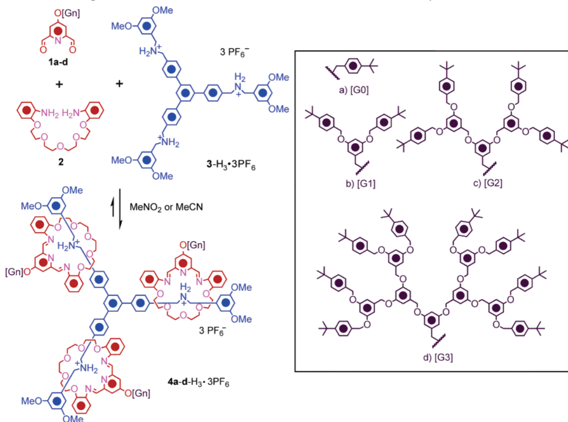
Scheme 2. Synthesis of the [G0]–[G3] Dendritic Dialdehydes 1a–d
