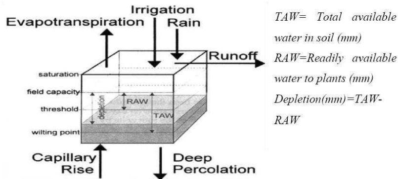
Figure 2 FAO-56 logic of soil water balance (adapted from Allen et al. [1998]).
