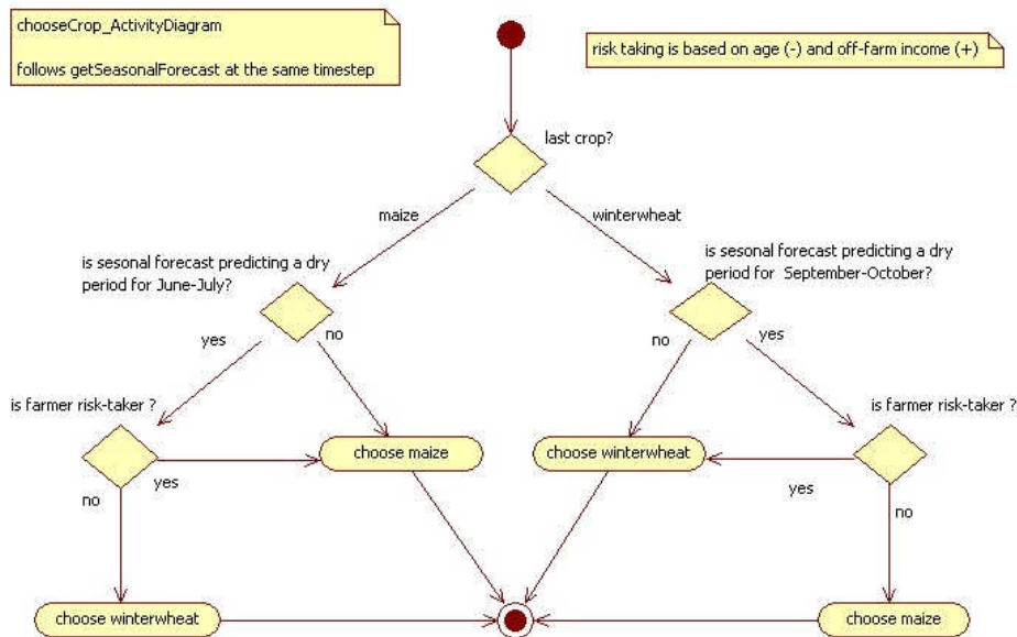
Figure 4 chooseCrop UML activity diagram.
