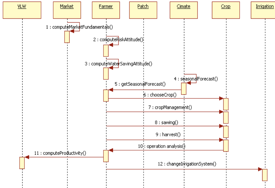
Figure 3 UML sequence diagram of strategic level.
