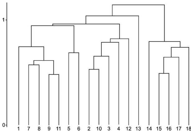
Figure 2. Dendrogram of the 18 relevés of Table I. Algorithm: complete link, chord distance; cover data.
