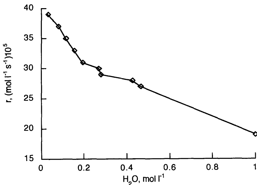
Fig. 7. Influence of the concentration of H 2 O on the initial reaction rate of hydrogenolysis of ethyl mandelate in ethanol. Run conditions as in Fig. 2, except for the concentration of [HCl]=0.0135 \text{ mol l}^{-1} .
