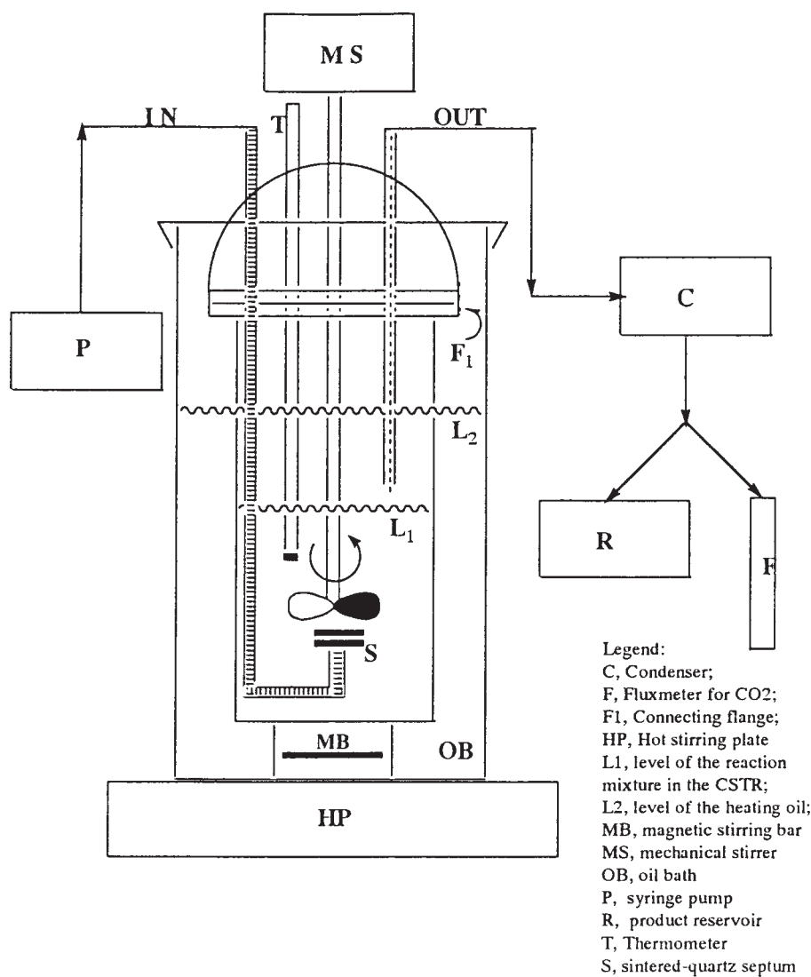
Fig. 3. CSTR reactor.
