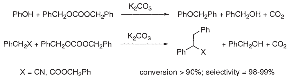
Scheme 15. Benzylation of phenol and \text{CH}_2 -active compounds with DBzIC.
