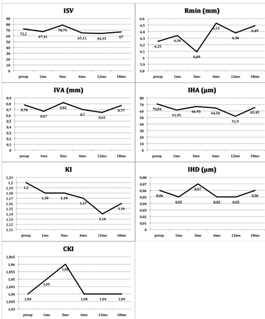
Figure 2. Change in topography indices over time after cross-linking. Index of surface variance (ISV), index of vertical asymmetry (IVA), keratoconus index (KI), central keratoconus index (CKI), minimum radius of curvature (Rmin), index of height asymmetry (IHA), index of height decentration (IHD).
