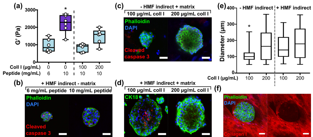
Fig. 10. Combined control of matrix additions and co-culture influences MCF10A organisation. (a) Box plots ( n = 6 ) showing bulk oscillatory rheology results of peptide gels with and without matrix modifications, *indicates p < 0.05 relative to all other conditions (one-way ANOVA), (b) acinar morphology on indirect co-culture with HMF, (c) acinar morphology in MCF10A monoculture in 10 mg/mL peptide gels with matrix additions, (d) acinar morphology on indirect co-culture with HMF in 10 mg/mL peptide gels with matrix additions, (e) quantification of acinar diameter for each condition, *indicates p < 0.05 relative to all other conditions (Kruskal-Wallis, >25 acini across 2 independent experiments per condition), (f) immunostaining of an acinus surrounded by collagen I matrix in a 10 mg/mL peptide gel modified with 200 \mu\text{g/mL} collagen I. Scale bar 50 \mu\text{m} .
