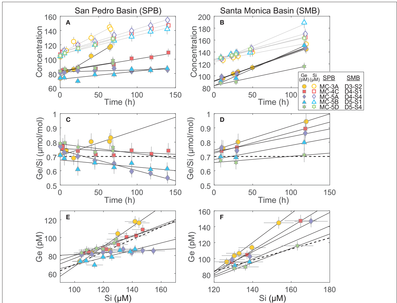
FIGURE 3 | Incubation results of cores from San Pedro and Santa Monica basins (SPB and SMB, respectively): (A,B) The increase of Ge and Si concentrations in the incubated overlying water. These slopes, once corrected for water loss via sampling (see Supplementary Data ), were used to determine the benthic Ge and Si fluxes reported in Table 3 ; (C,D) The change in the Ge/Si ratio of the overlying water. The thick dashed line shows the Ge/Si of biogenic silica in the SPB and SMB sediments ( 0.7 \mu\text{mol/mol} ; Baronas et al., 2016); (E,F) plots showing Ge vs. Si concentration over the course of the incubations. These slopes were used to calculate the benthic flux Ge/Si ratio ( Table 3 ). The thick dashed line shows Ge/Si of biogenic silica ( 0.7 \mu\text{mol/mol} ).
