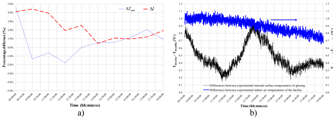
Figure 2. a) Values of \Delta T_{amb} and \Delta I , b) differences between T_{int,clear} and T_{int,milky} as well as between T_{indoor,clear} and T_{indoor,milky} as a function of the time.
