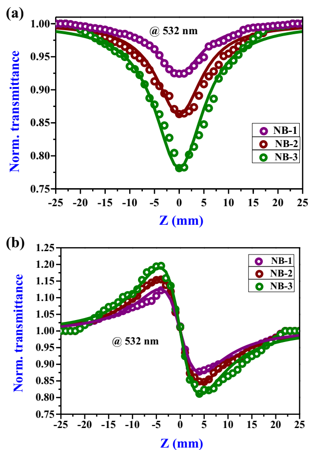
Fig. 3 Z-scan signatures of gold doped NB glasses using ns pulses and 532 nm excitation. a OA Z-scan data, b CA Z-scan data. Open circles represent the experimental data, while solid lines are theoretical fits
