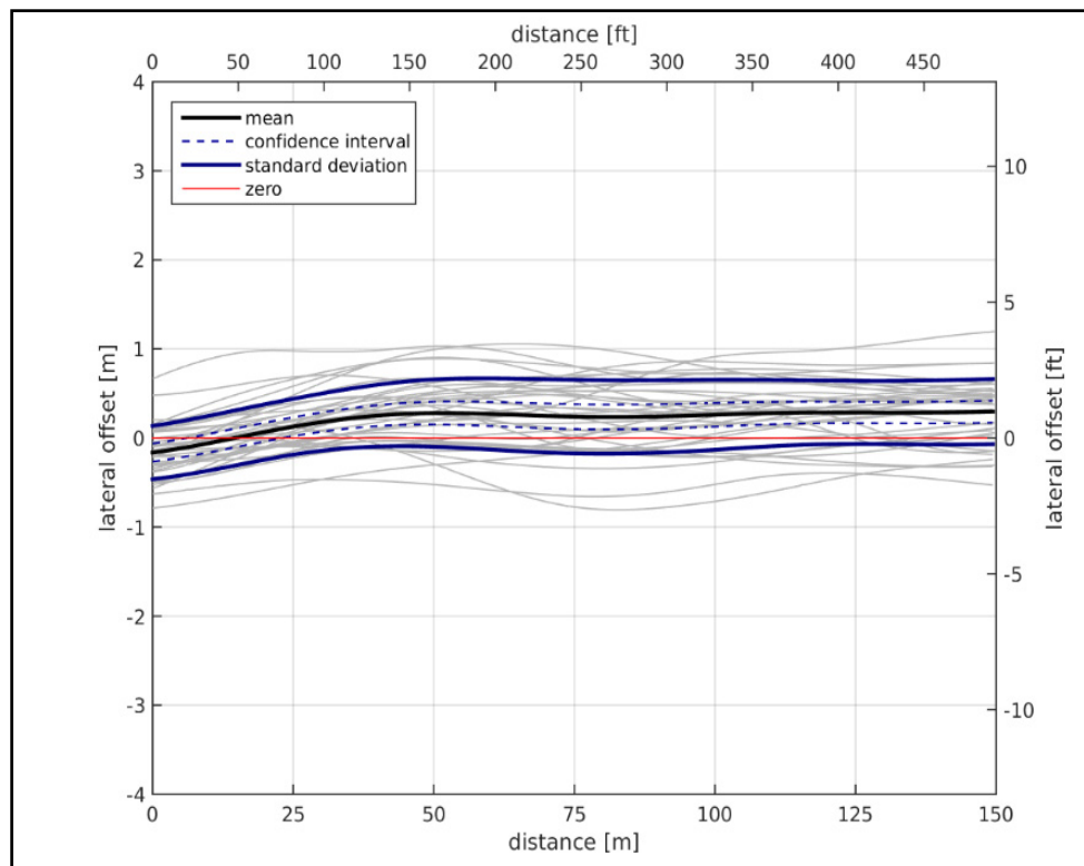
Figure 25. Observed Trajectories During the First 150 Meters (~500 ft) of the S-Curve for the Manual Drive Baseline
