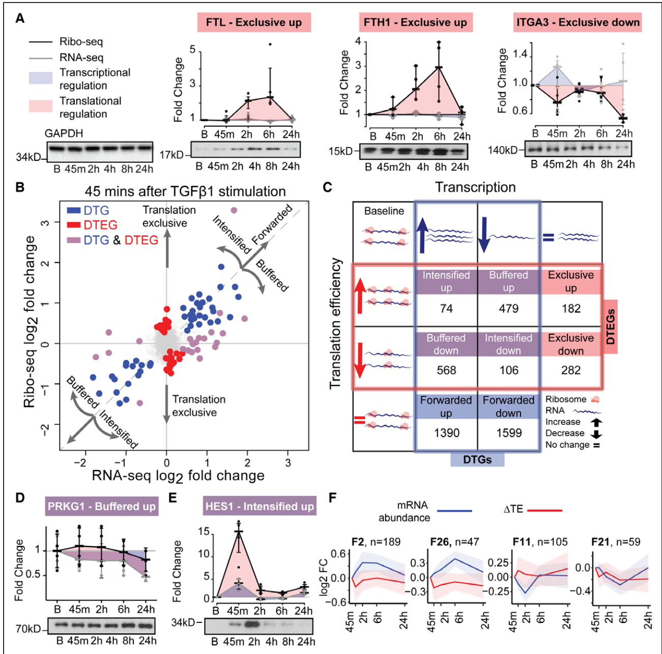
Figure 3. Genome-wide temporal transcriptional and translational landscape in cardiac fibrosis.
