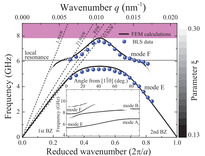
FIG. 5. Dispersion relation of SAWs propagating [1\bar{1}0] direction of a 1D surface phononic crystal. BLS experimental data (full circles) compared with FEM calculations (lines). Dotted lines show the corresponding dispersion relations of longitudinal (L BAW), transverse (T1 BAW and T2 BAW) bulk waves, and Rayleigh (RSW) surface waves typical for Si. The inset presents the calculated angular dispersion of SAWs at q = 0.0105 \text{ nm}^{-1} .
