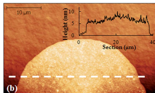
Fig. 4 (a) Optical image of the \mu -SQUID susceptometer taken after depositing sample DPN2 . (b) AFM topography image of a deposit formed on \text{Si}/\text{SiO}_2 under identical conditions to those used for sample DPN2 and (inset) cross-section recorded along the white dashed line in image (b).
