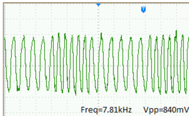
Figure 25. FSK Signal Obtained between the Left Earphone Channel and the Ground
