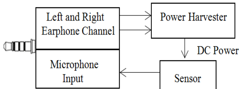
Figure 4. Block Diagram Windoo Smartphone Sensing Platform
