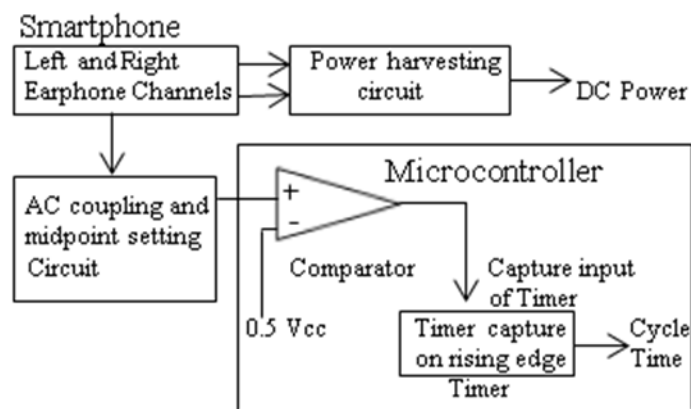
Figure 14. Block Diagram of the Joint Power Harvesting and Communication Technology
