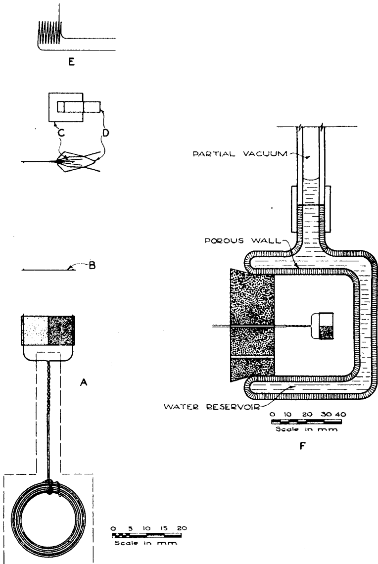
Fig. 1. Bismuth antimony thermojunction for measuring relative humidity.
