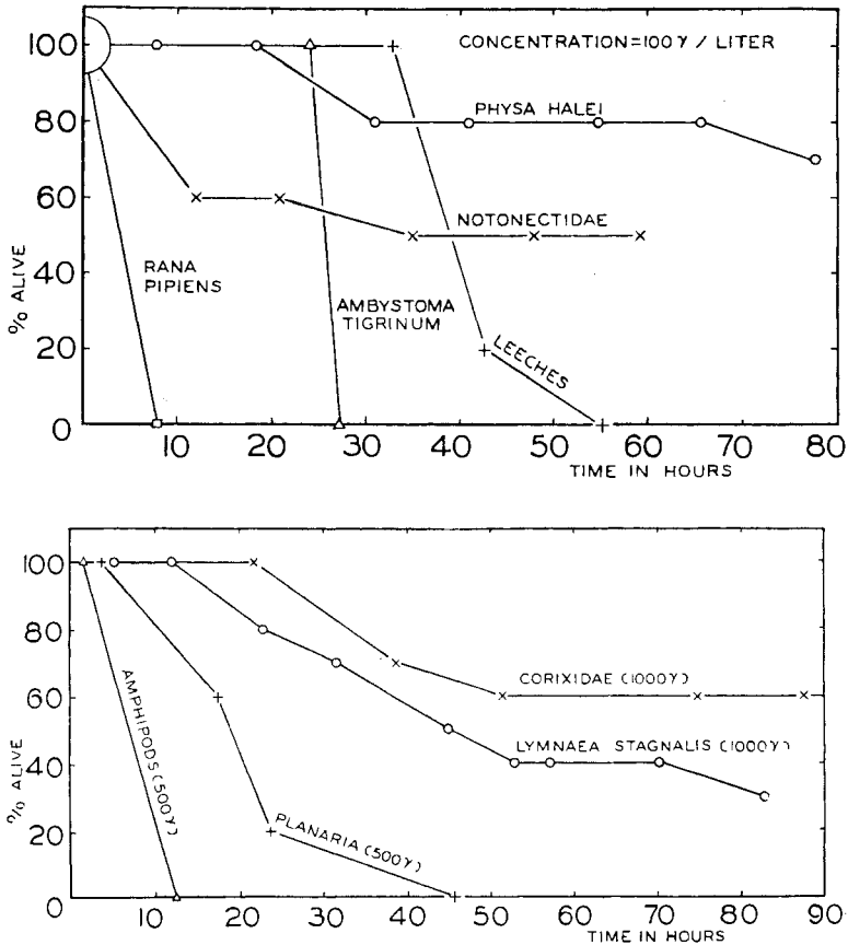
Fig. 2. Responses of animals to high concentrations of rotenone. Note that a certain percentage of more resistant individuals can live beyond the effective period of the poison (2-3 days).
