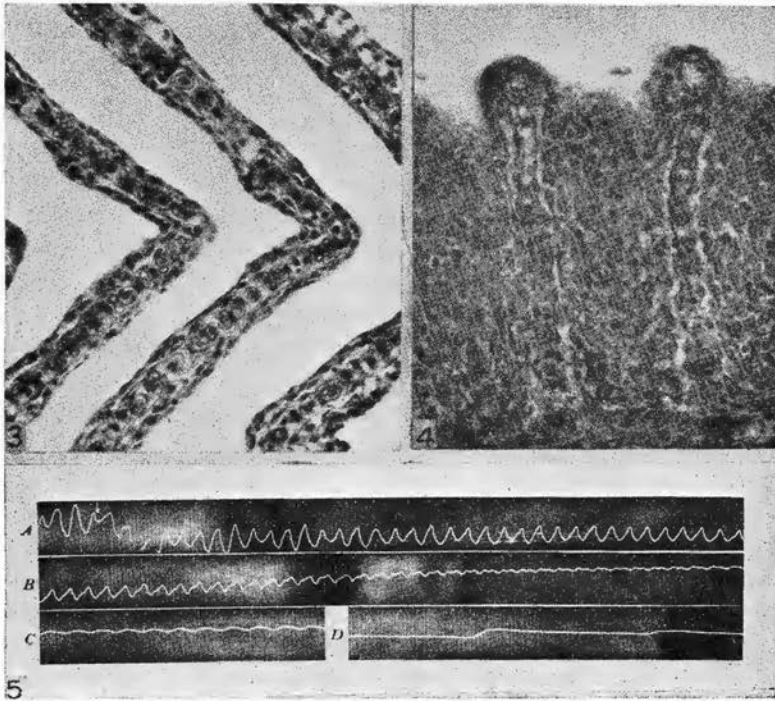
Fig. 3. Transverse section of gills from an untreated bullhead. Note the large number of erythrocytes within the capillaries.
