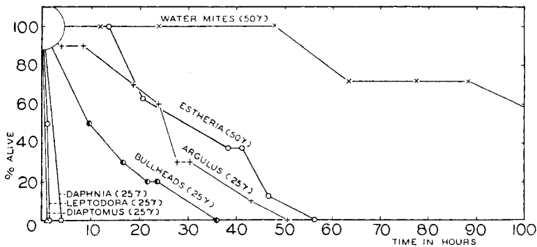
Fig. 1. Susceptibilities of various animals to dilute concentrations (expressed as \sqrt{1.} ) of rotenone.
