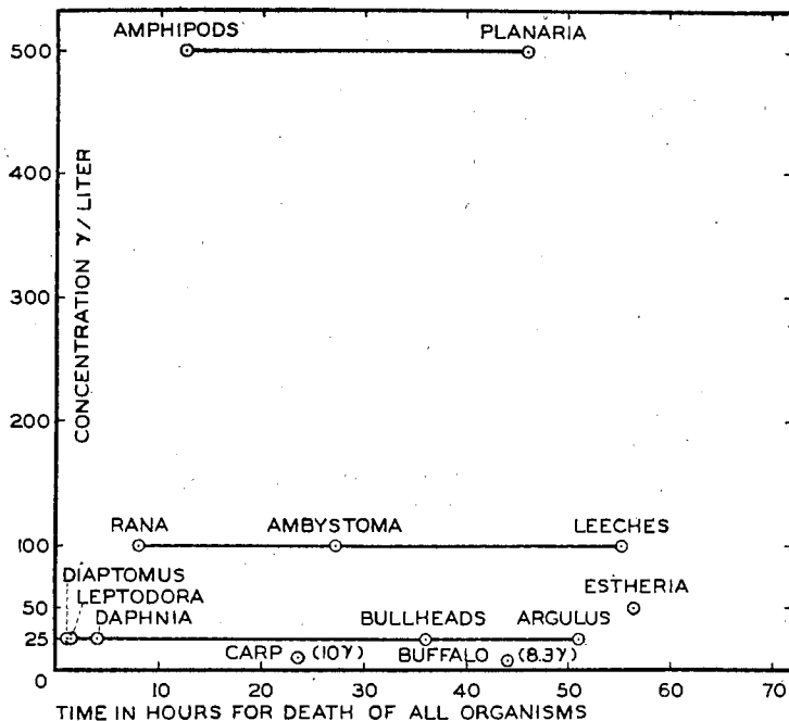
Fig. 6. Order of sensitivity of fresh water animals to rotenone with respect to lethal concentrations of the drug and time of death. The graph should be read from right to left and from top to bottom. Thus, Planaria are the least sensitive and Buffalo the most sensitive. At any single concentration level, the nearer the point lies to the ordinate, the more sensitive is the organism (i.e., less time is required for death of all individuals).
