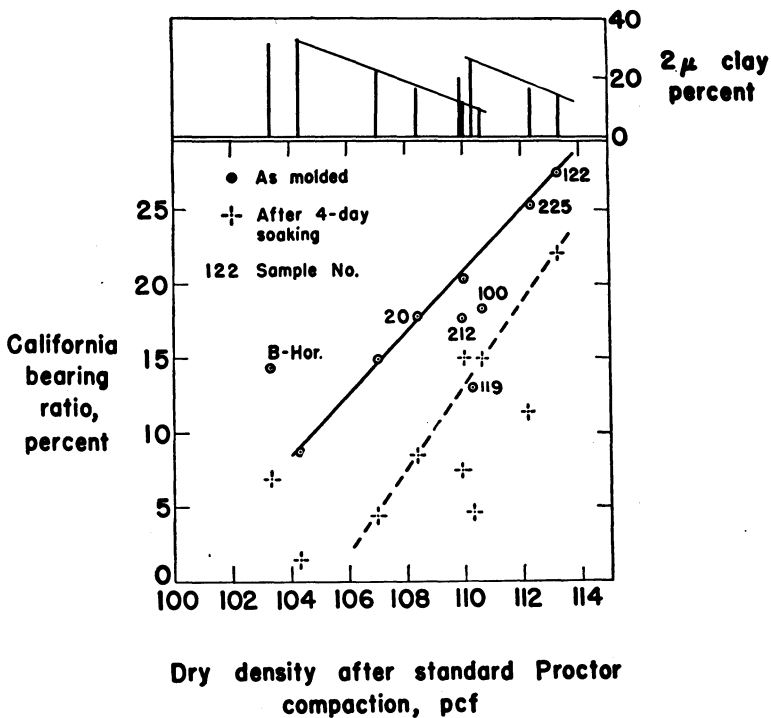
Figure 11. California Bearing Ratio related to compacted density. There are two points for each sample, since the C.B.R. is lowered by soaking. Graph at the top shows the clay content of each sample.
