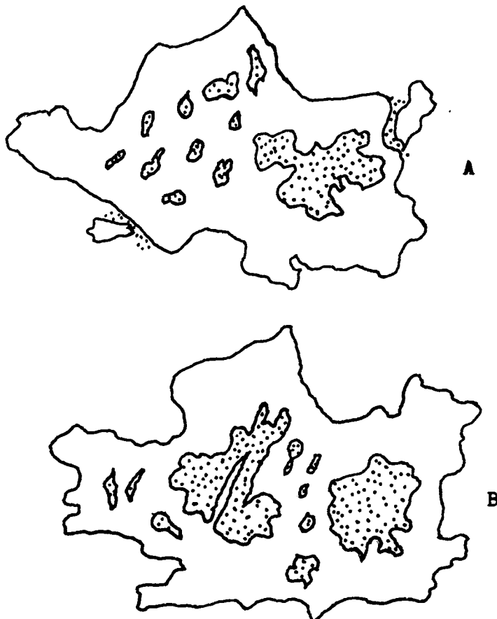
Figure 1. Camera lucida sketch of a single calcite crystal containing pellets. "A", before etching "B", after a thirty-second etch with 1N acetic acid. Stippled, pellet material; plane, matrix calcite.
