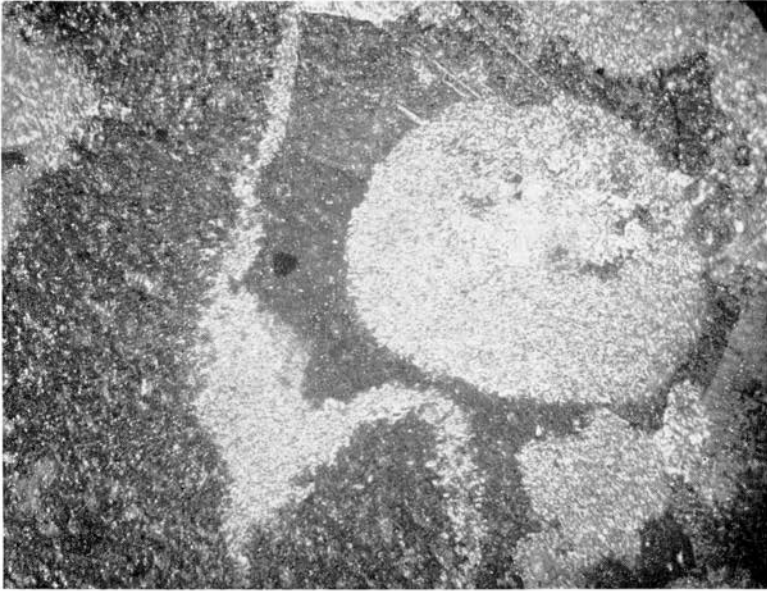
Figure 5. Single crystal of matrix peikilitically enclosing a pellet and partially replacing another. Crossed nicols, 155x.
