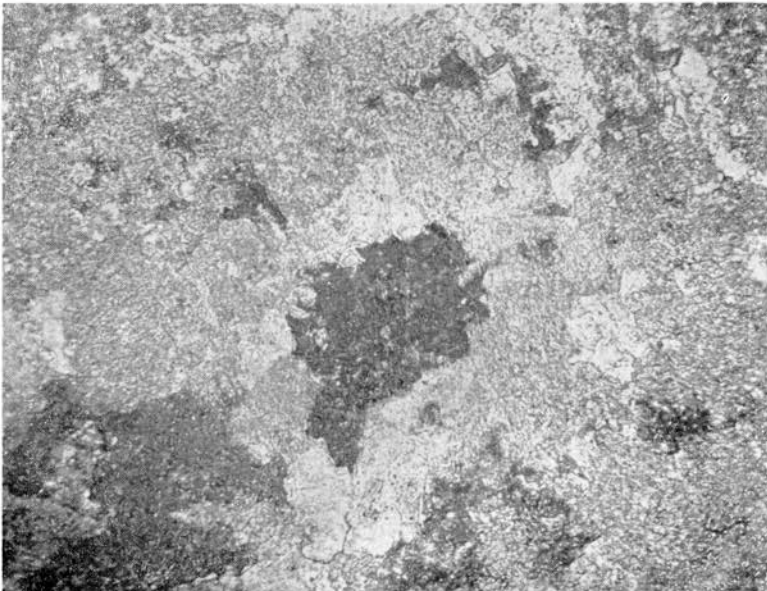
Figure 6. Partially re-crystallized pellet fragments in a crystal of matrix calcite. Crossed nicols, 155x.
