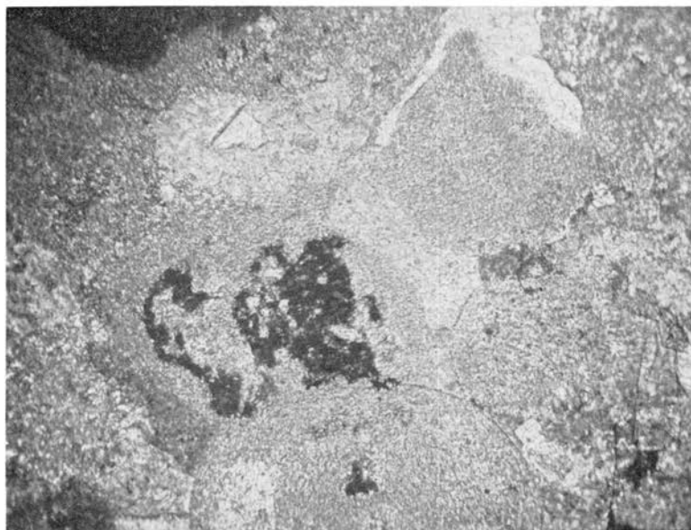
Figure 3. Pellets showing inclusions of irregular coarse calcite. Light areas are matrix calcite, gray areas are pellets, and black area is an inclusion in the central pellet. Crossed nicols, 155x.
