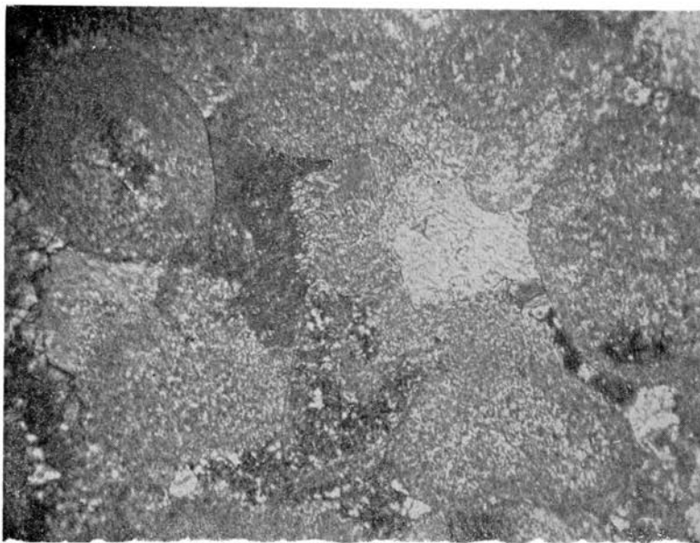
Figure 4. Boundary relationships of pellets against matrix calcite. Crossed nicols, 155x.
