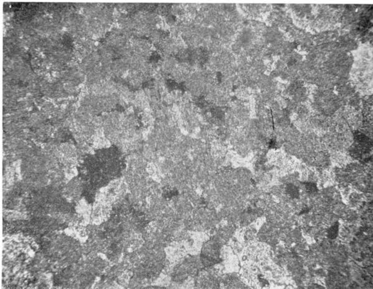
Figure 2. General textural relationships in the Gilmore City limestone. Indistinct gray masses, pellets; light areas and black patches, matrix calcite. Crossed nicols, 79x.
