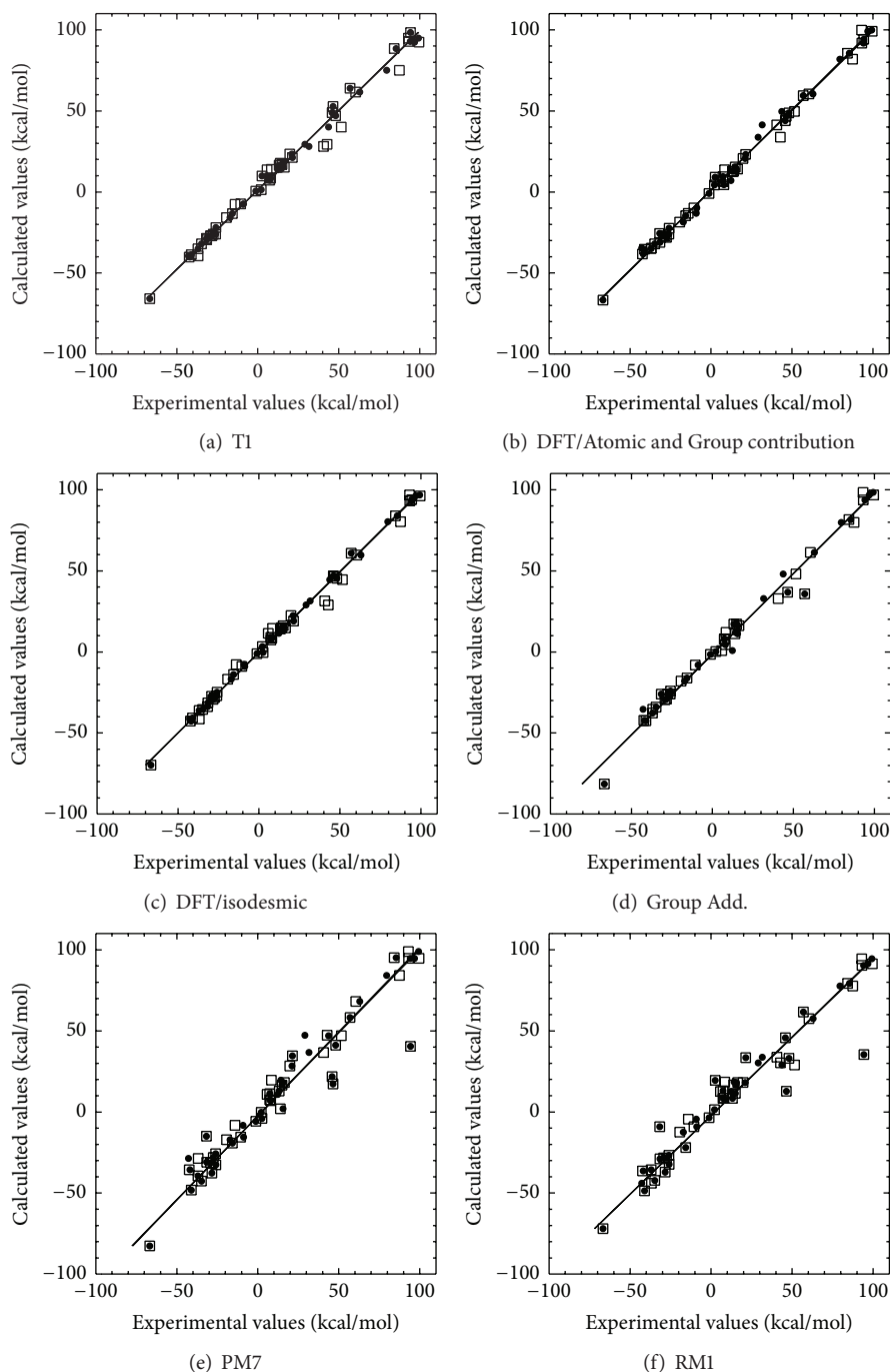
FIGURE 1: Calculated gas-phase heat of formation values versus experimental values. Gas-phase heat of formation values were calculated using (1) the multilevel ab initio approach (T1) described by Ohlinger et al. [8] as implemented in the Spartan'10 and 14 suite of programs (a); (2) the DFT/Atomic and Group contribution approach developed and described by Byrd and Rice [6, 7] (b). The experimental values and calculated values used to construct (b) are those published by Byrd and Rice [6, 7]. (b) is identical to Figure 1a in their manuscript except for the fact that the alternative set of experimental \Delta_f H_{298,g}^o reference values are also included. (3) Density functional theory using isodesmic, isogyric, and other balanced equations as described herein (c). (4) The Benson Group Additivity approach as implemented in the NIST and CHETAH 8.0 software programs (d); (5) semiempirical theory (PM7 and RM1) as implemented in MOPAC2012 and the Spartan 14 suite of programs ((e) and (f), resp.). Open squares represent calculated \Delta_f H_{298,g}^o values versus the experimental \Delta_f H_{298,g}^o values. Closed circles represent calculated \Delta_f H_{298,g}^o values versus the alternative experimental \Delta_f H_{298,g}^o reference values as described in the text. Least square regression analysis and calculation of R^2 values were accomplished using KaleidaGraph graphing software (Synergy Software, Reading, PA). R^2 values are presented in Tables 2 and 3.
