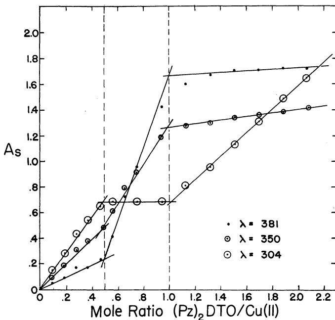
Figure 2. Mole ratio plot for the copper (II)- (Pz)_2DTO system.
