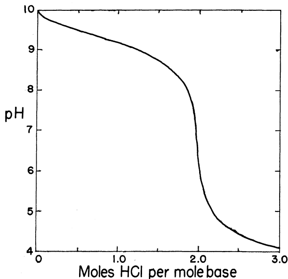
Figure 1. Titration of .01 M (Pz)_2 DTO with .01 M HCl.
