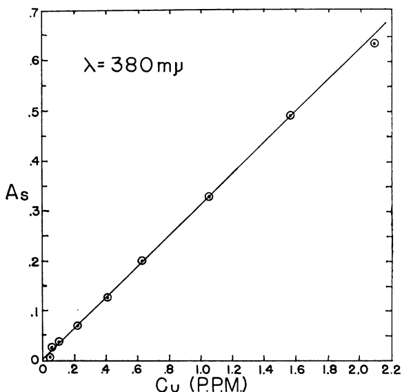
Figure 3. Calibration curve for the determination of copper (II) with (Pz)_2DTO .
