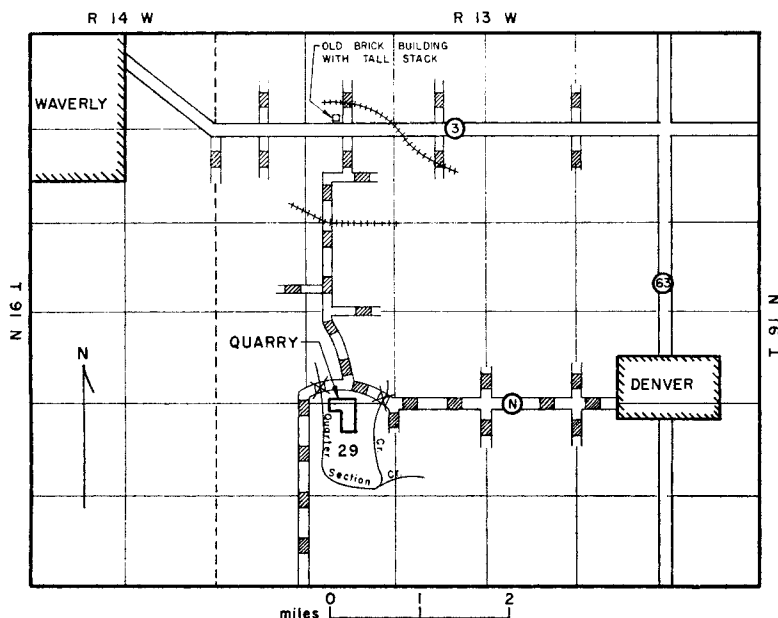
FIG. 1— LOCATION MAP OF DENVER QUARRY
