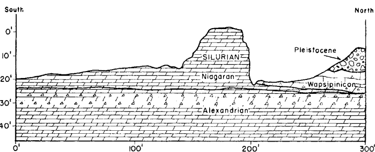
Fig. 4—Diagram of west wall of quarry showing large Silurian hummock with Devonian beds deposited on and adjacent to the eroded surface.
