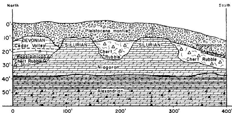
Fig. 5—Diagram of east wall of quarry showing two Silurian hummocks with Devonian beds deposited on and adjacent to the eroded surface.
