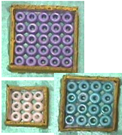
Figure 4. Sets of donuts in boxes to illustrate Z=n^2 .
