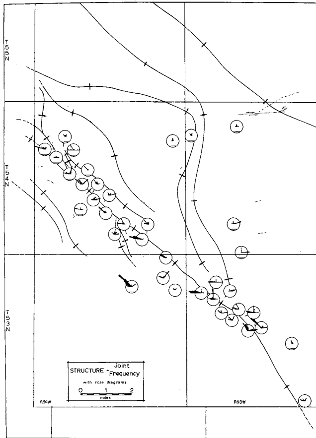
Figure 7 Map showing joint frequencies at selected points of study with relation to structural axes.
