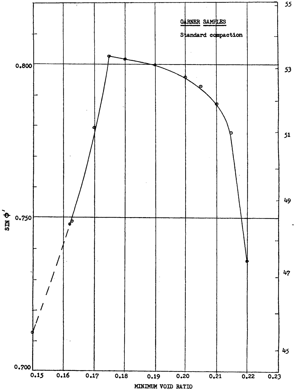
Figure 7. Garner stone: values of \sin \phi' and \phi' as related to minimum void ratio.
