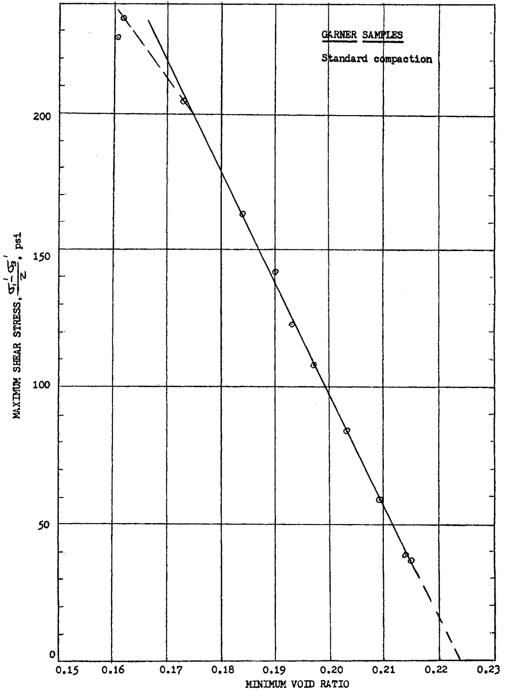
Figure 5. Garner Stone: maximum shear stress as related to minimum void ratio
