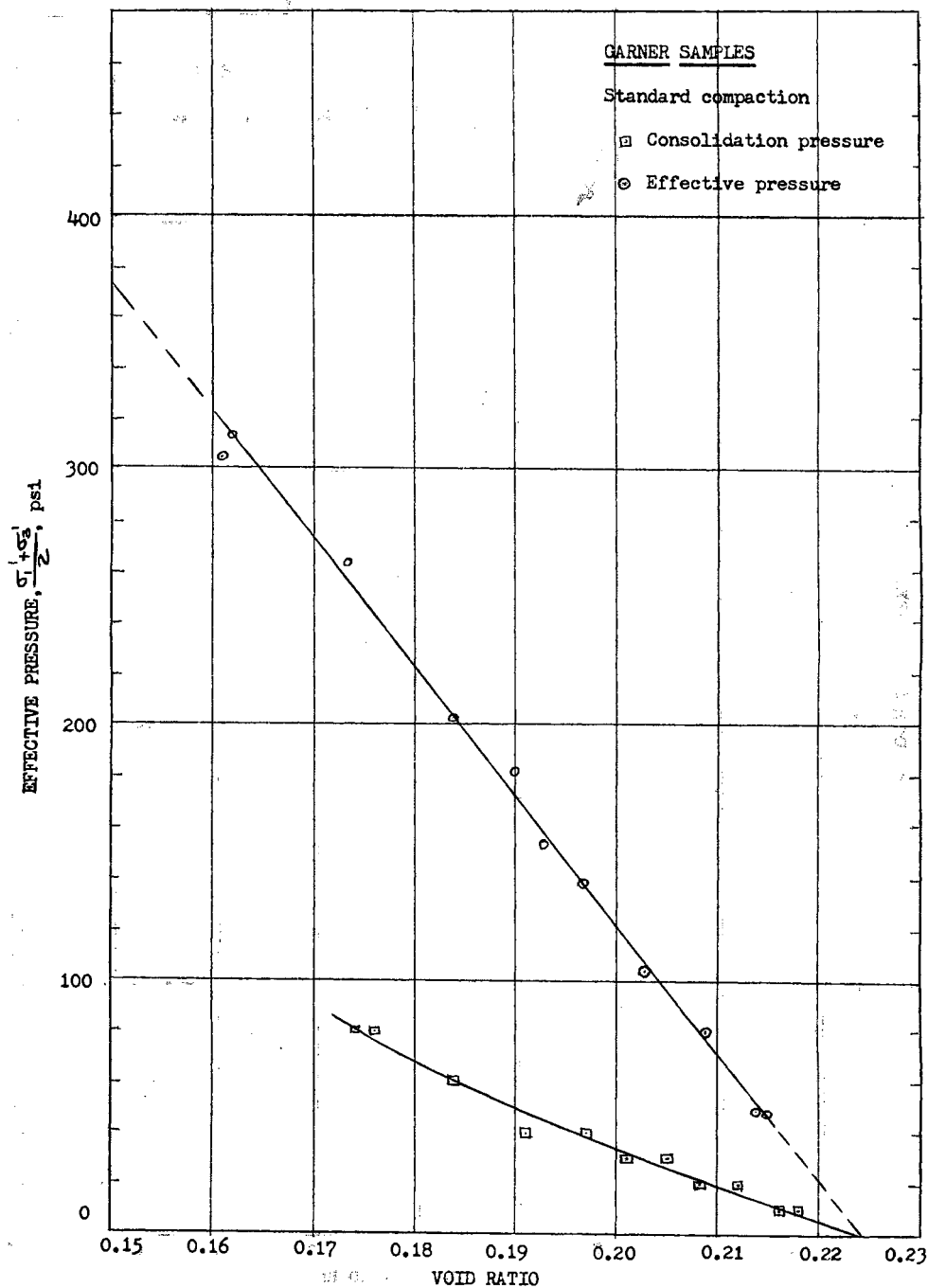
Figure 6. Garner stone: effective pressure and consolidation pressure as related to void ratio.
