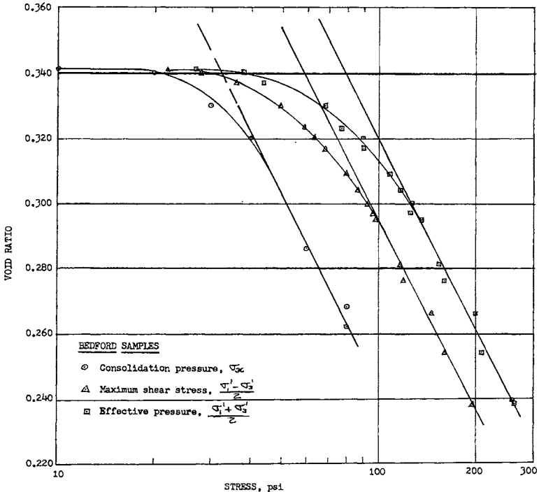
Figure 1. Bedford stone: consolidation pressure, maximum shear stress, and effective normal pressure as related to void ratio.
