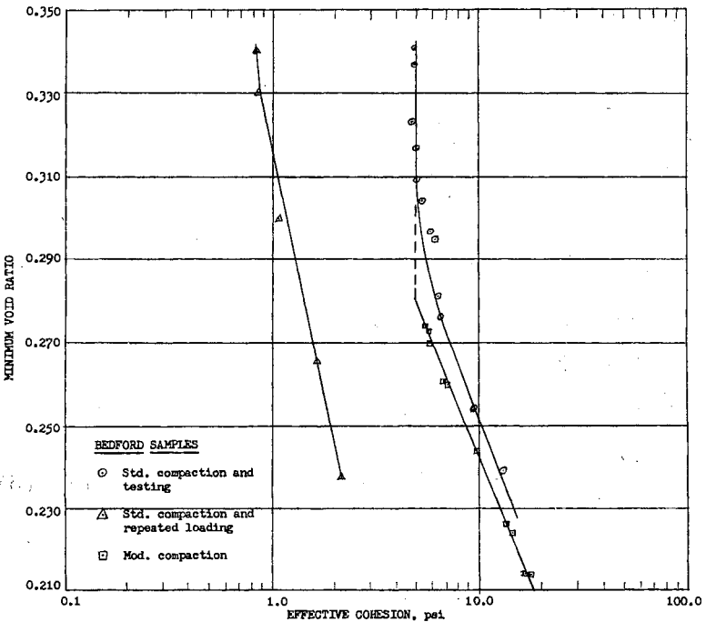
Figure 4. Bedford stone: relationship between the minimum void ratio and the effective cohesion.
