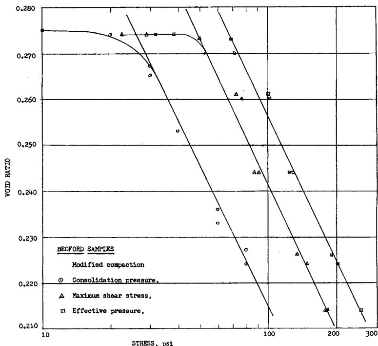
Figure 2. Bedford stone. consolidation pressure, maximum shear stress, and effective normal pressure as related to void ratio.
