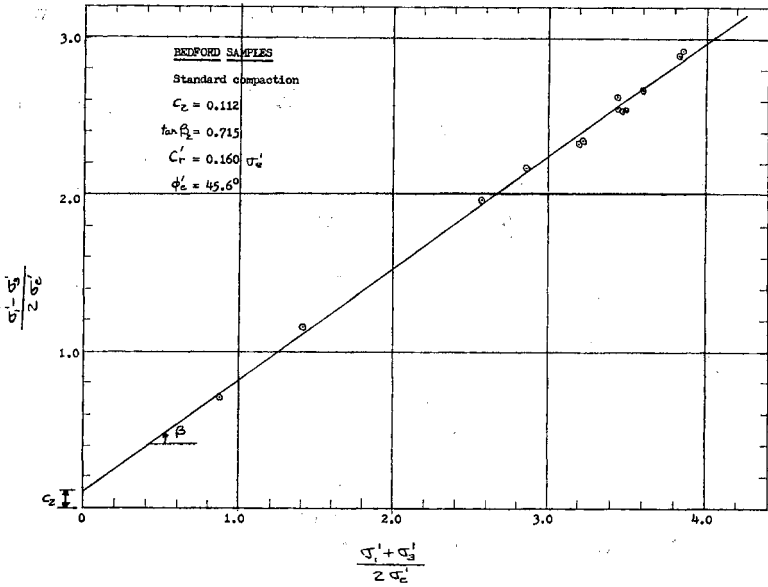
Figure 3. Bedford stone: relationship between \sigma'_1 - \sigma_3 and \frac{\sigma'_1 + \sigma_3}{2\sigma'_c} .
