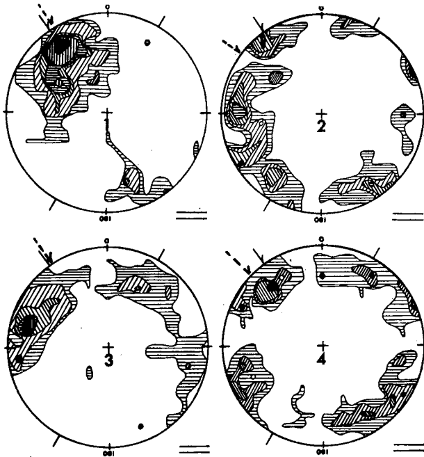
Figure 5—Fabric diagrams for site 1, 3¾ miles west of Garden City. Striae trend shown with an arrow in fourth quadrant. Ridge axis is shown by the two marks outside the first and third quadrants. Dashed arrow indicates mean fabric azimuth. Zero degree (top) is north.
