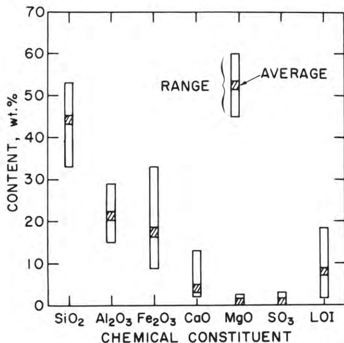
Figure 2. Range and average content of different chemical constituents in United State fly ashes (5, 6).
