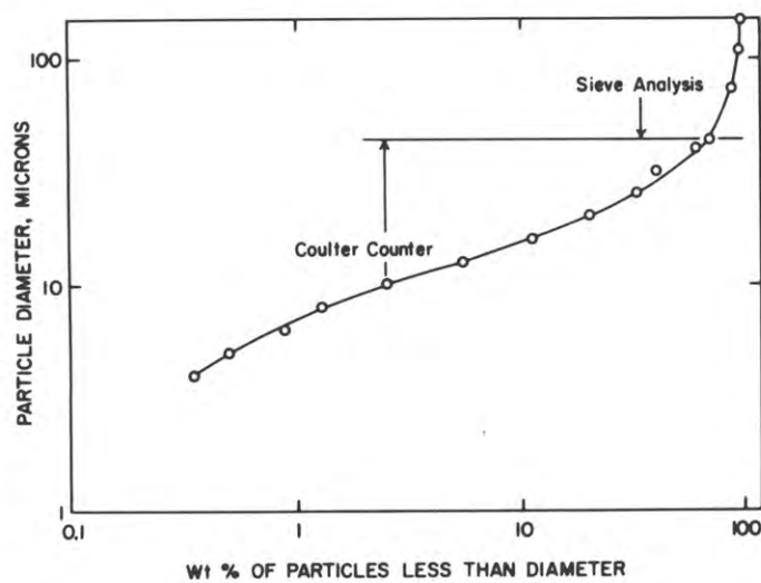
Figure 4. Size analysis of the magnetic fraction of fly ash.
