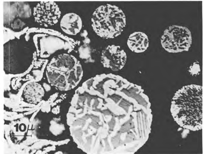
Figure 6. Photomicrographs of the cross-sections of particles from the magnetic fraction of fly ash.
