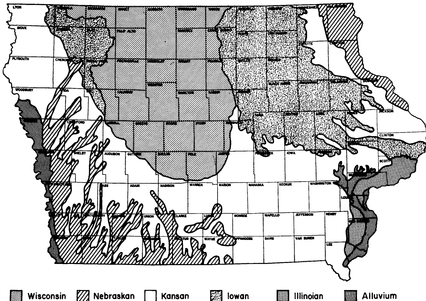
Fig. 1. Glaciation of Iowa.
