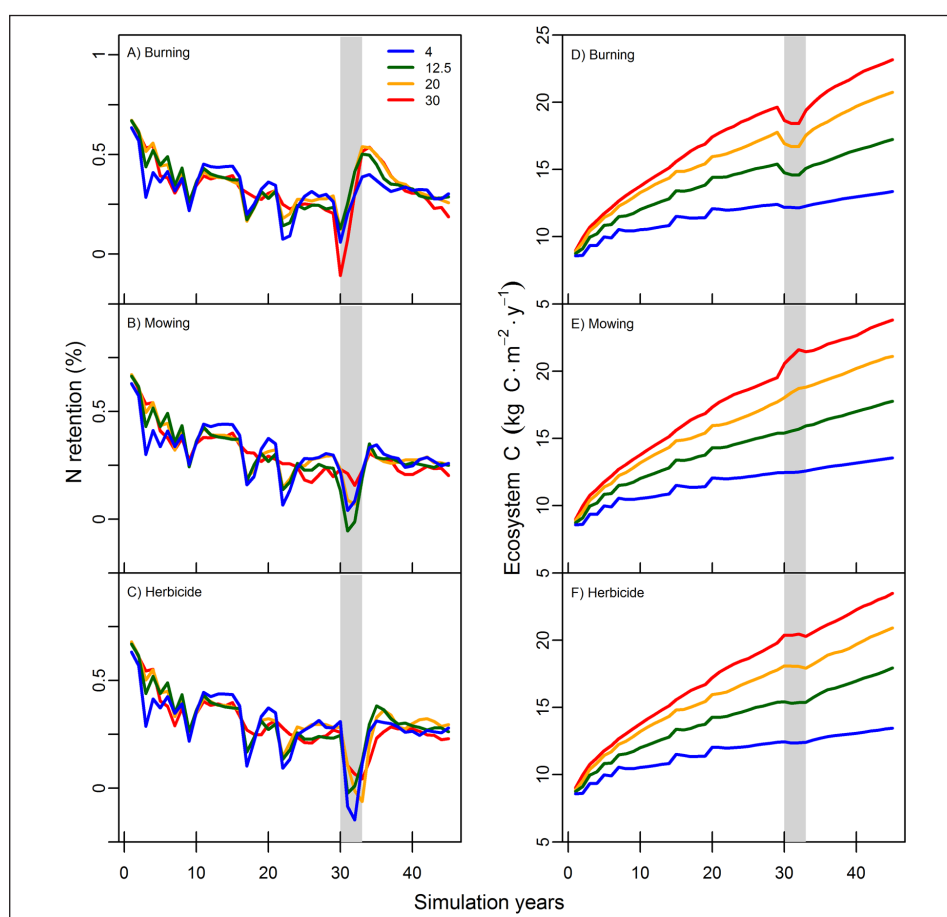
Figure 4: N retention and C accumulation in managed wetland simulations. The percent of incoming N retained (a–c) and amount of C accumulated (d–f) in the wetland over 45 simulation years. Wetlands received 4 (blue), 12.5 (green), 20 (yellow) or 30 (red) \text{g N} \cdot \text{m}^{-2} \cdot \text{y}^{-1} . Gray shading indicates the 3-year time period during which burning (a, d), mowing (b, e), or herbicide treatments (c, f) were applied. DOI: https://doi.org/10.1525/elementa.147.f4
