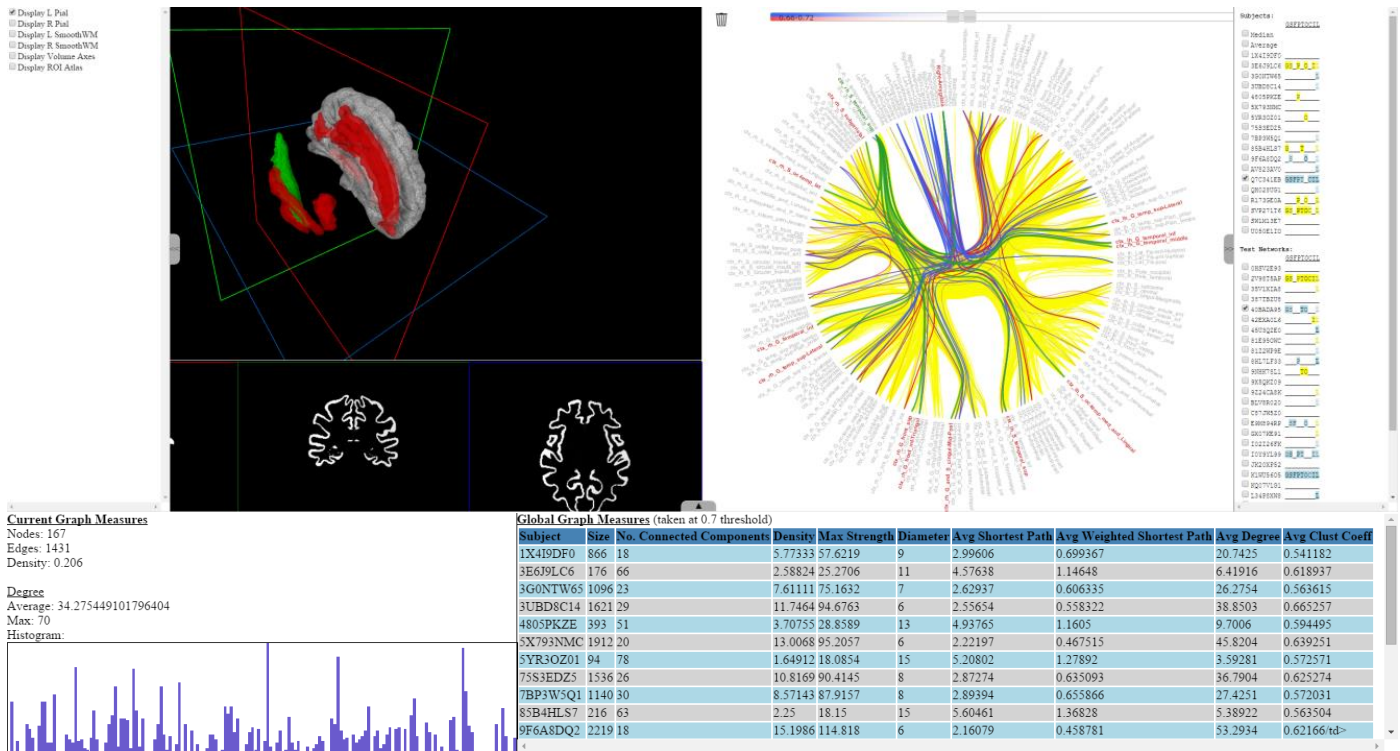
Fig. 1. Overview of the CereVA interface comparing two fMRI correlation networks: 3D rendering and volume display on the left; network abstraction on the right; statistical network analysis at the bottom. On the rendering, the green area is the selected node while the red ones are the correlated regions, within the current threshold. On the radial network abstraction, yellow background edges are highly similar, high correlation edges; blue and red edges are correlations within the specified threshold where blue edges have a higher correlation in the first subject's network and red in the second; green edges show the correlations for the selected node, which match nodes highlighted in the 3D rendering on the left. This image is from our previous study in [13].
