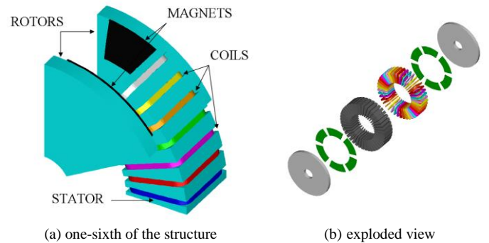
Fig. 1 Conventional TORUS AFPM
