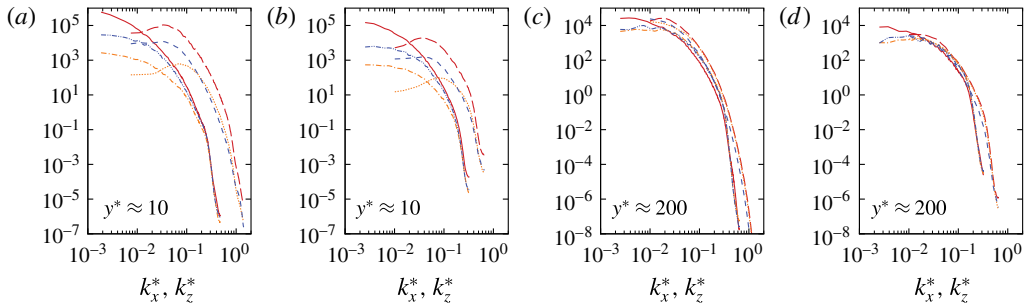
FIGURE 22. (Colour online) One-dimensional spectra for cases AM3R7 ( a,c ) and PM1R3 ( b,d ), at y^* \approx 10 ( a,b ) and y^* \approx 200 ( c,d ). — (red) E_{\rho uu}^{(x)}/\tau_w ; - - - (red) E_{\rho uu}^{(z)}/\tau_w ; ····· (orange) E_{\rho vv}^{(x)}/\tau_w ; ····· (orange) E_{\rho vv}^{(z)}/\tau_w ; - · - · (blue) E_{\rho wv}^{(x)}/\tau_w ; - - - (blue) E_{\rho wv}^{(z)}/\tau_w .
