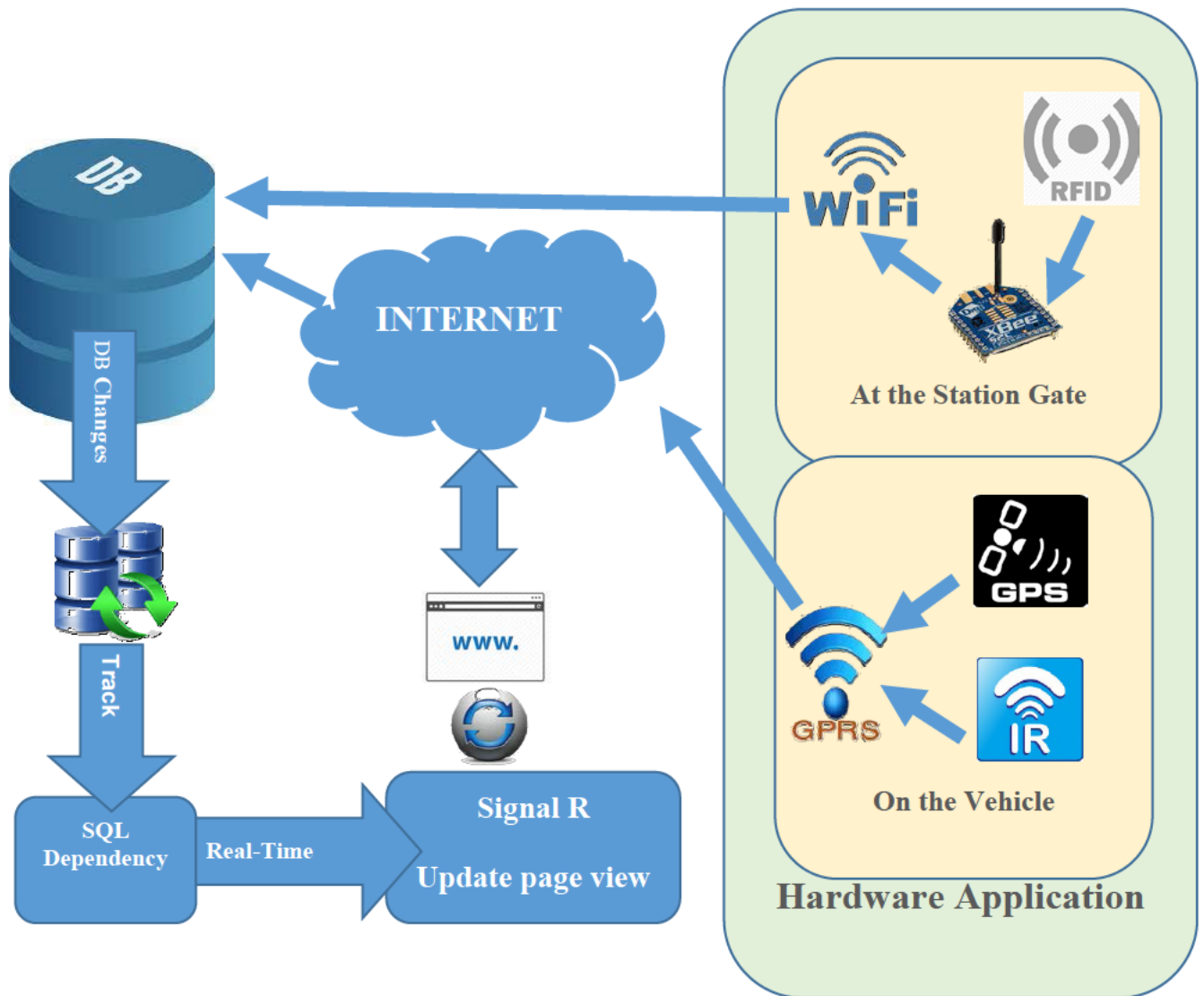
Figure 5-12: Framework Architecture
