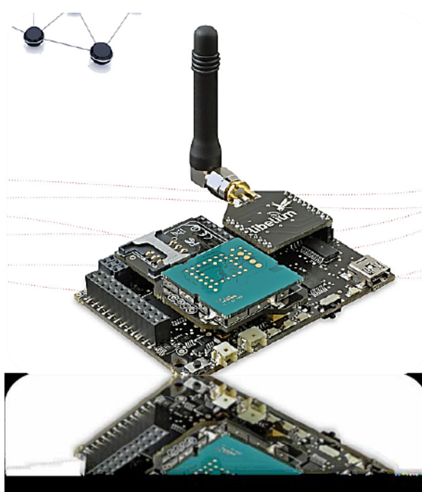
Figure 5-11: Wasp mote Board with GPS, GPRS and Wi-Fi (Libelium, 2017)
