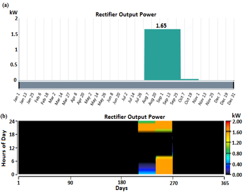
Fig. 10: Rectifier output power (a) maximum power (b) hourly power (Case 2)
