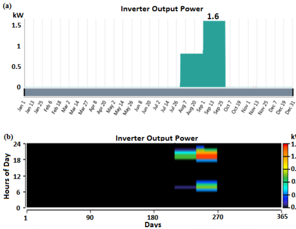
Fig. 6: Inverter output power (a) maximum power (b) hourly power (Case 1).
