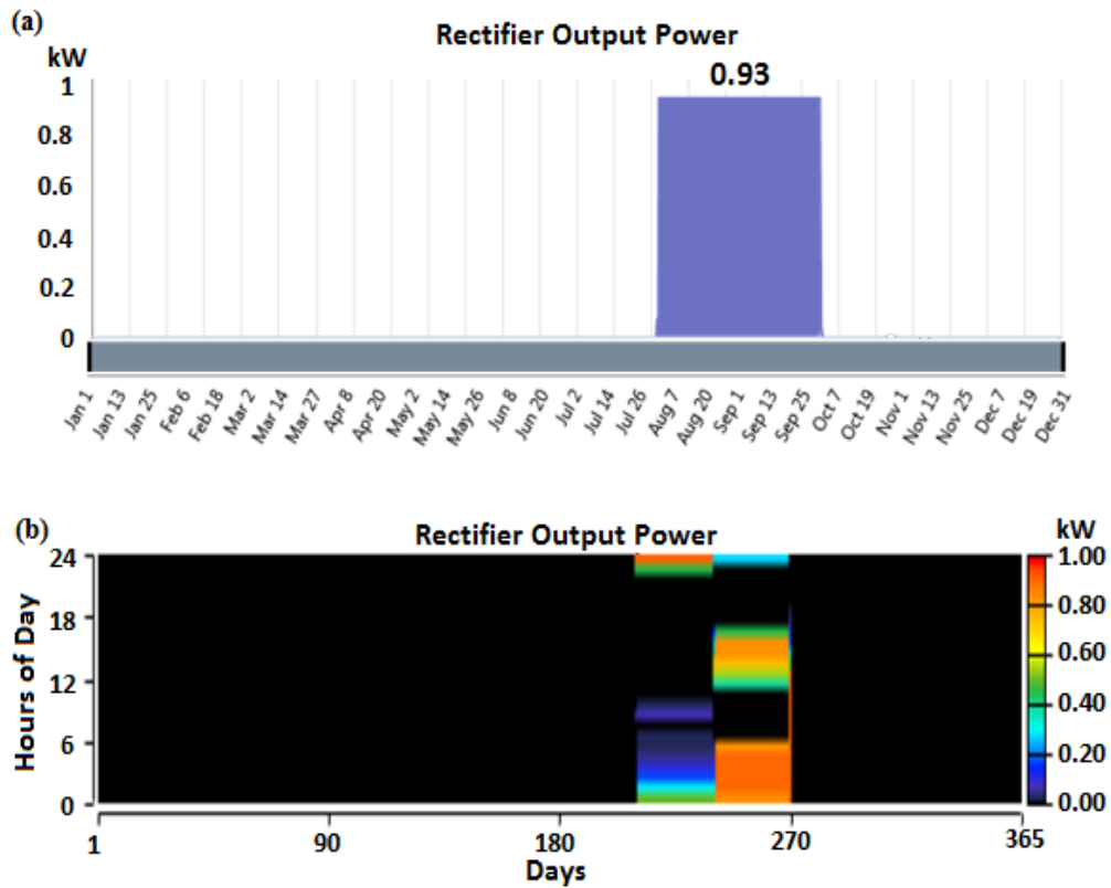
Fig. 7: Rectifier output power (a) maximum power (b) hourly power (Case 1)
