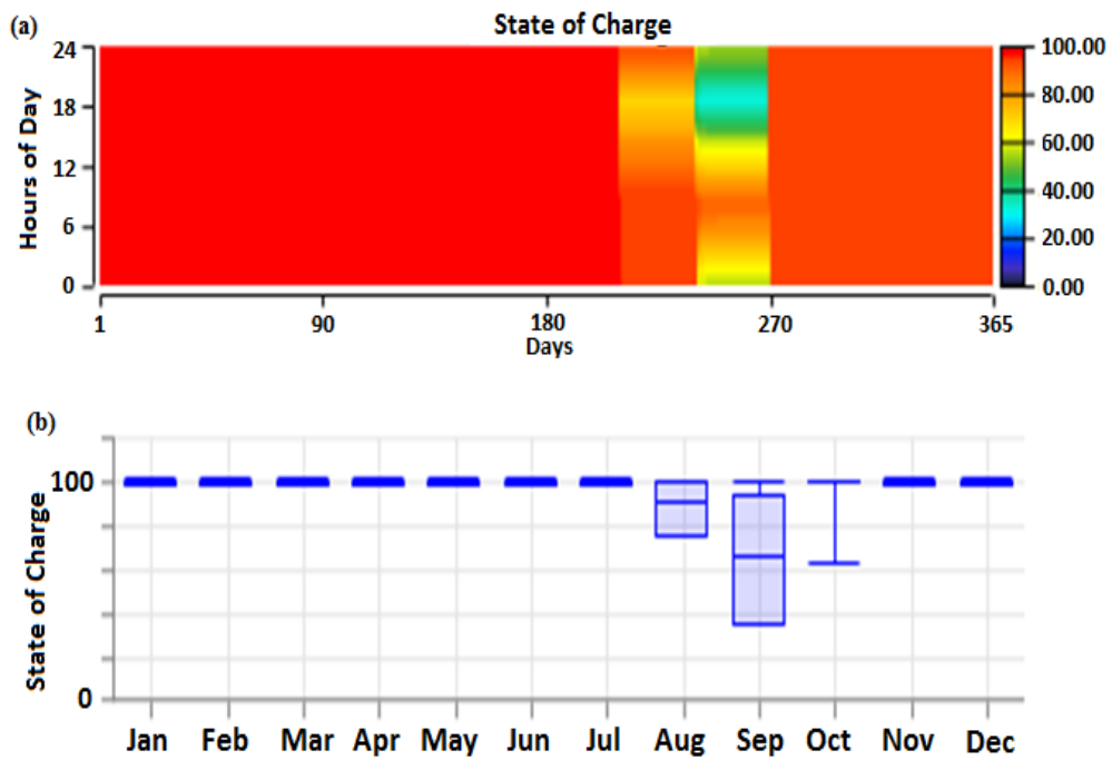
Fig. 11: Batteries state of charge (a) hourly (b) monthly statistic (case 2)
