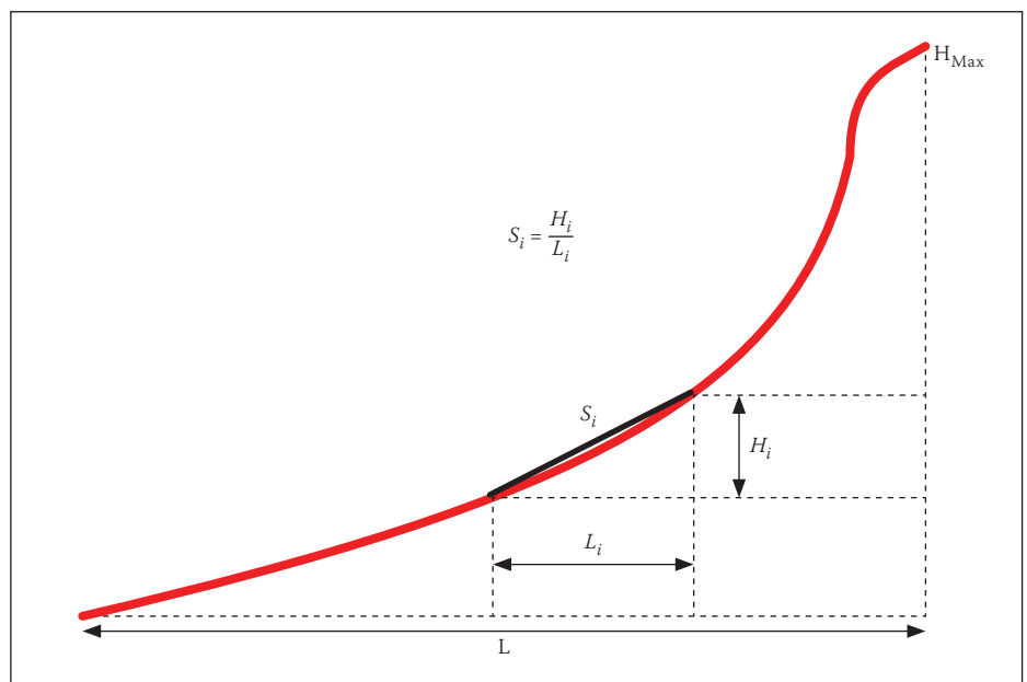
Figure 6 Taylor-Schwarz method (Gericke 2010)
