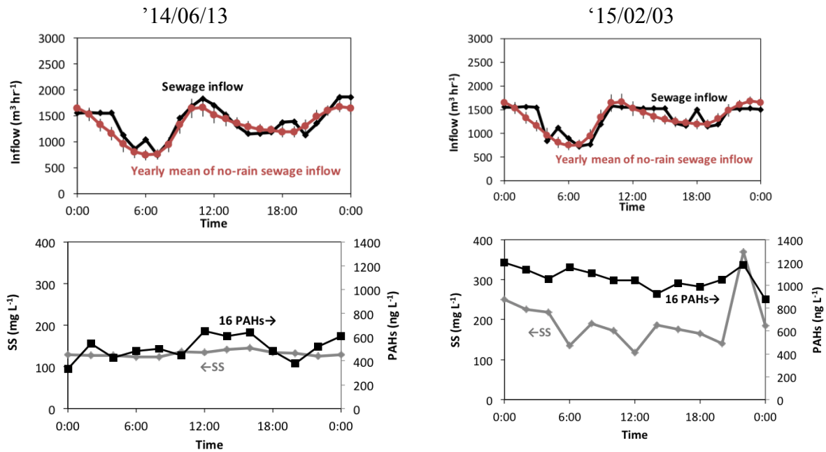
Fig. 3. Diurnal changes of Sewage inflow, SS, and 16 PAHs concentrations during no-rain periods
