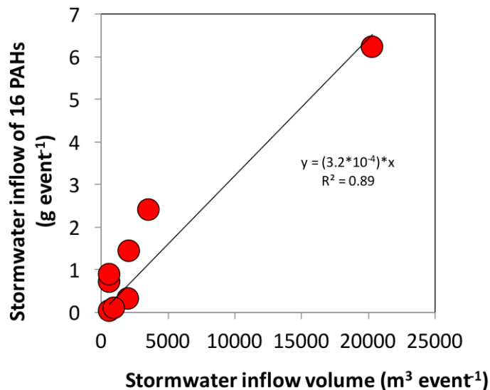
Fig. 6. Relationship between stormwater inflow volume and 16 PAHs
