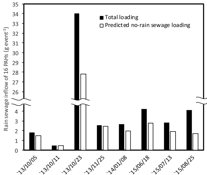
Fig. 5. Sewage inflow loading of PAHs for each rainfall
