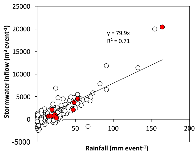
Fig. 2. Relationship between rainfall and stormwater inflow (12/04/01–16/03/31; Red circles denote the events of PAHs sampling)
