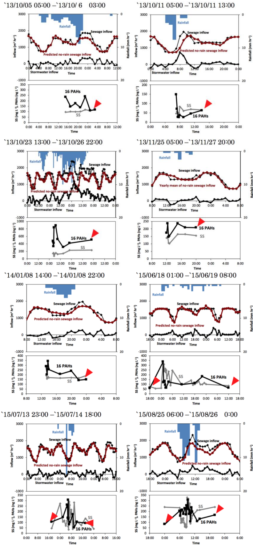
Fig. 4. Sewer inflows during rainfalls (Red arrows indicate the samplings that are used for no-rain PAHs concentrations for the rains)
