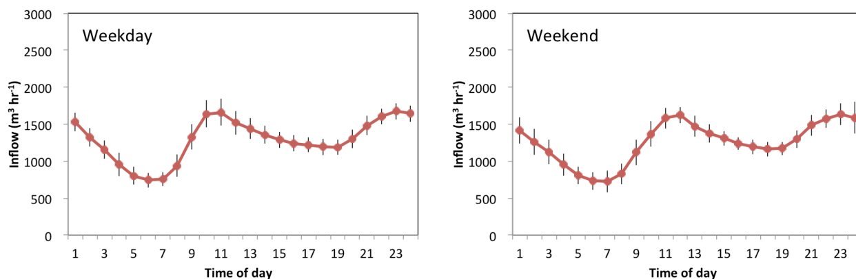
Fig. 1. Yearly mean of sewage inflow volume during no-rainfalls (April 1, 2014–March 31, 2015, \pm bars represent standard deviation)
