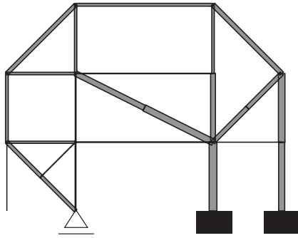
Figure 4: Optimal configuration of Type 1 for Problem P1 with stress constraints.
