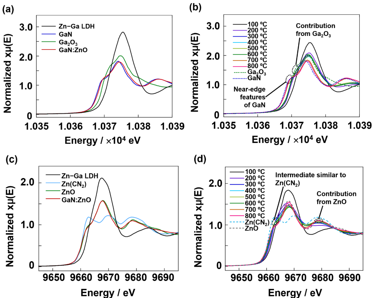
Figure 7. (a, b) Ga K-edge and (c, d) Zn K-edge ex-situ XANES spectra of samples. Spectra of standard samples (Zn-Ga LDH, GaN, Ga_2O_3 , Zn(CN_2) , ZnO, and GaN:ZnO) are given in (a) and (c). Spectra of mixtures of Zn-Ga LDH and urea heat-treated at 100, 200, 300, 400, 500, 600, 700, and 800 °C are given in (b) and (d).
