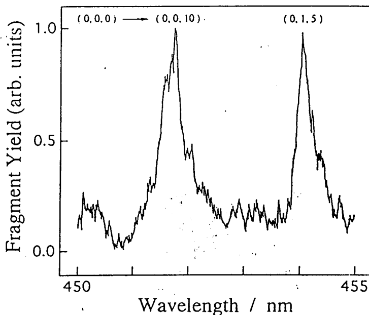
Fig. 2. Photodissociation spectrum of \text{CH}_3\text{I}^+ .
