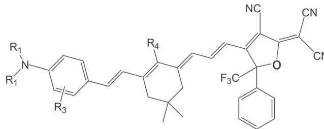
FIG. 2. Molecular structure of dipolar phenyltetraene chromophore for SEO100.
