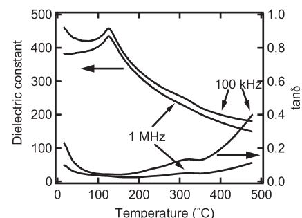
FIG. 2. Temperature dependence of the dielectric constant and loss tangent of the BT-KN composite.
